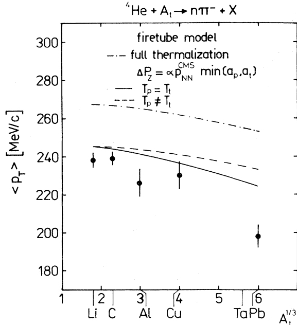
FIG. 3. Average transverse momenta \langle p_T \rangle of negative pions vs the target mass number A_t^{1/3} . Experimental points from Ref. 8.
