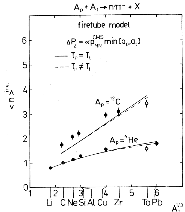
FIG. 2. Caption as for Fig. 1.
