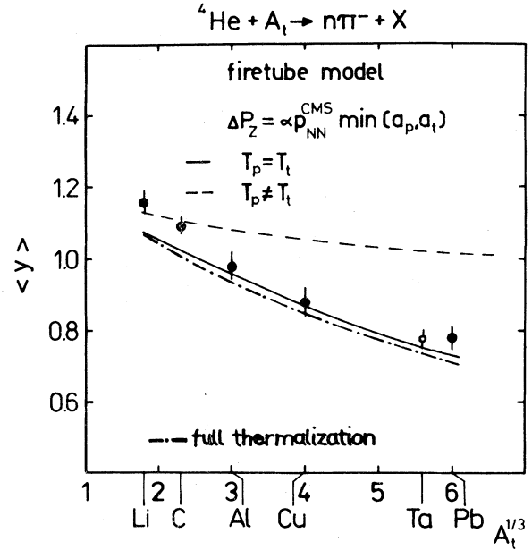
FIG. 4. Average rapidity \langle y \rangle of negative pions vs target mass number A_t^{1/3} . Experimental points (●) from Ref. 8 and (○) Ref. 12.
