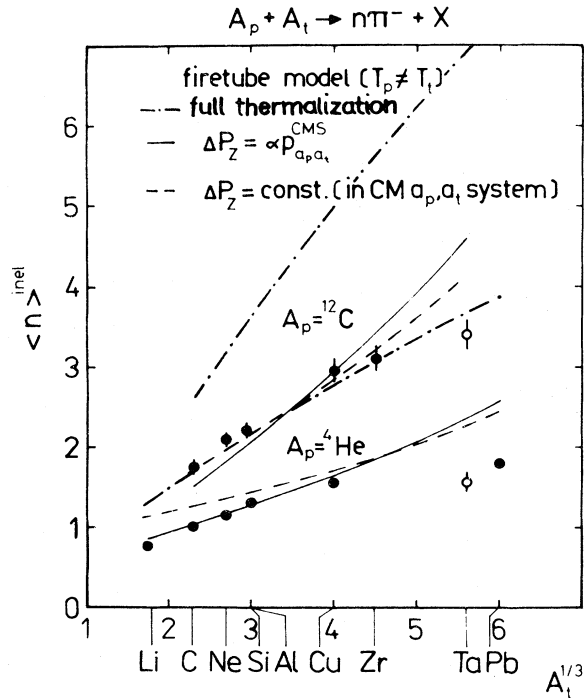
FIG. 1. Average multiplicities \langle n \rangle^{inel} of negative pions (normalized to \sigma^{inel} ) vs the target mass number A_t^{1/3} . Experimental points (●) from Ref. 7 and (○) from Ref. 9.
